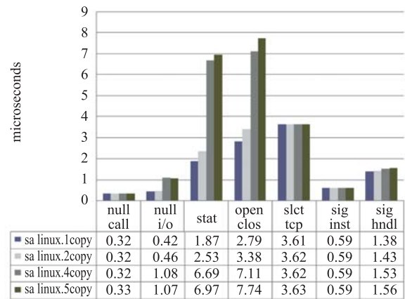
Figure. 6 Scalability of sa Linux process
