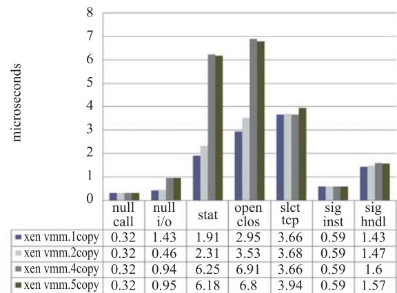
Figure. 7 Scalability of Xen VMM process
