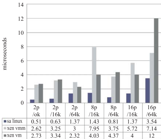
Figure. 4 Time overhead of context switching
