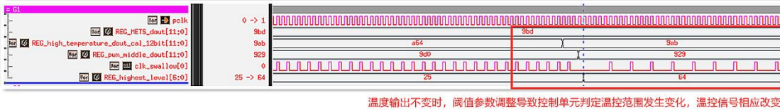
图 12 系统兼容性测试波形图 Fig.12 Waveform of system compatibility test
