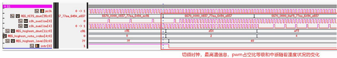
图 11 温度控制功能验证波形图 Fig.11 Waveform of temperature control function verification
